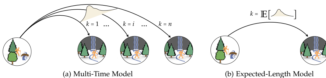
Figure 7.1: An intuitive illustration of the MTM (left) and ELM (right).
